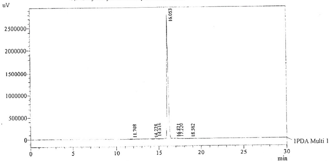
Chromatogram 3,2'-Dihydroxychalcone D:\promonence\Data
